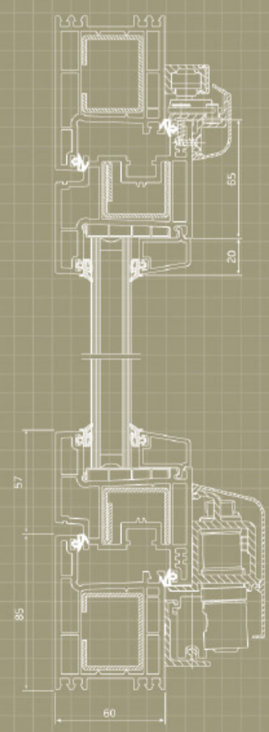
VERTICAL SECTION <A-A>
